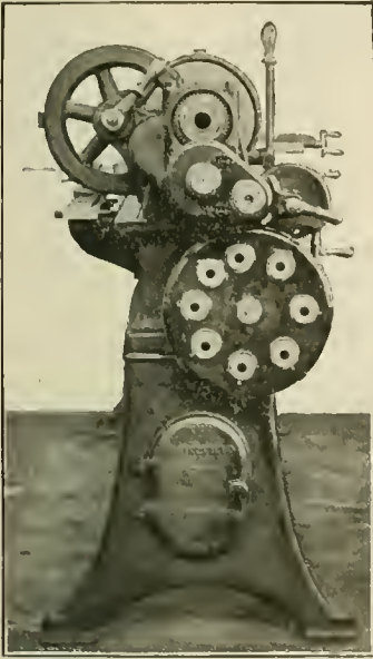
END VIEW SHOWING GEAR-CHANGING DEVICE.
